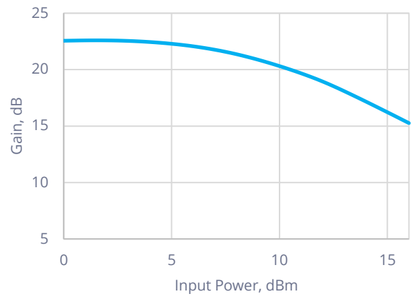
Gain, vs. Input power at 34 GHz
