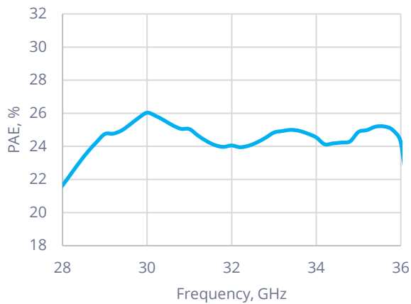
P.A.E. at ( P_{IN} = 10 dBm)
