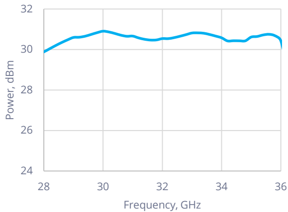
Output Power, at Pin=10 dBm
