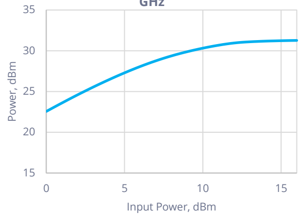
Output power vs. Input Power at 34 GHz
