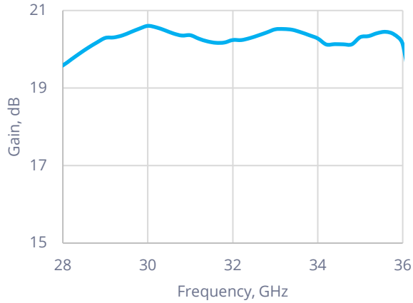
Small Signal Gain, at Pin=10 dBm
