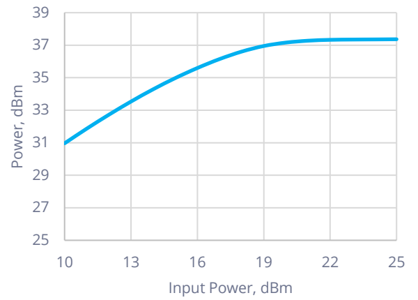
Power Output vs. Input at 34 GHz
