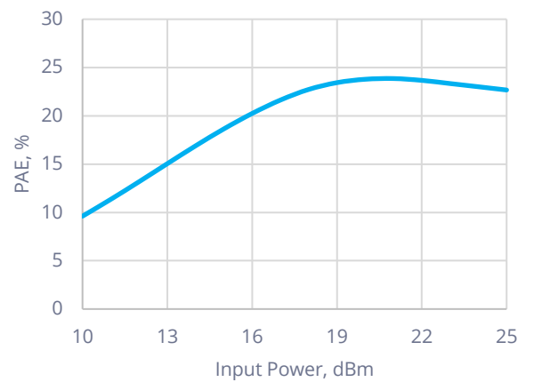
P.A.E. vs. Input Power at 34 GHz
