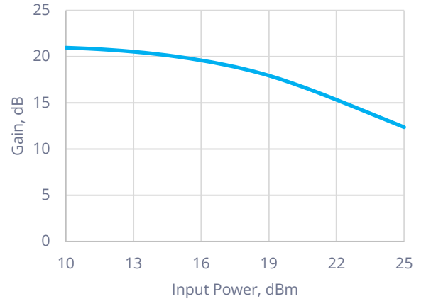
Gain vs. Input Power at 34 GHz
