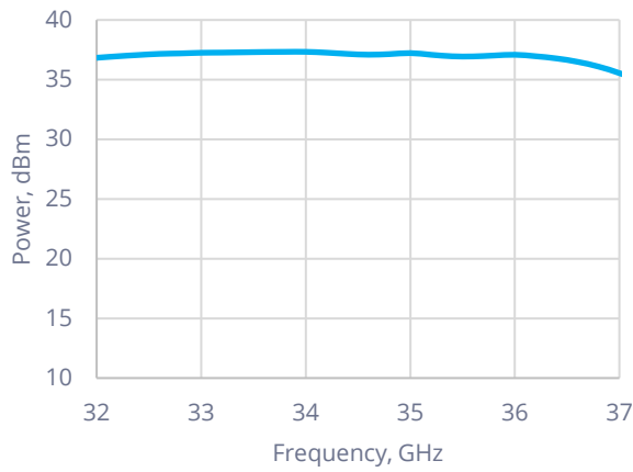
Output Power
