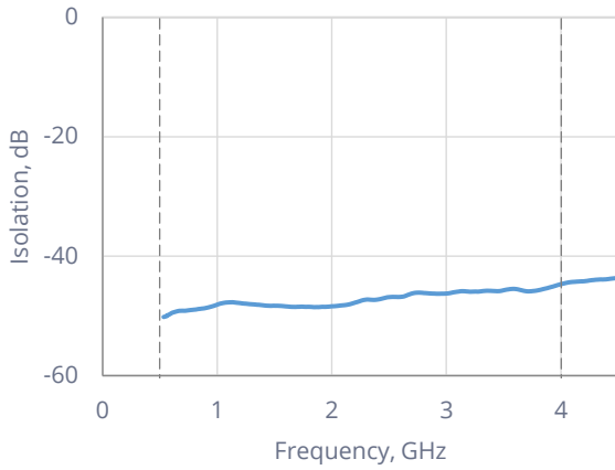
Reverse Isolation (On)
