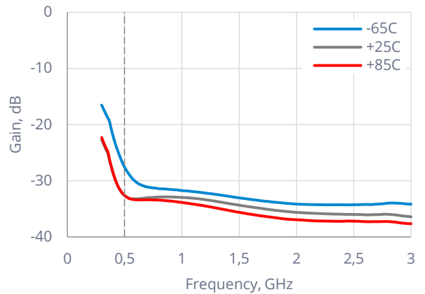
Small Signal Gain (Off)
