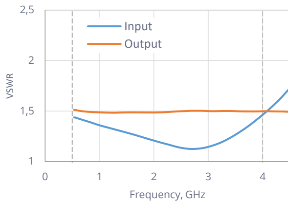
Voltage Standing Wave Ratio (On)
