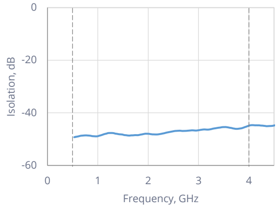
Reverse Isolation (Off)
