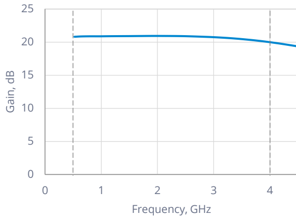
Small Signal Gain (On)
