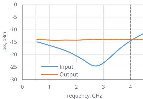
Return Loss (On)
