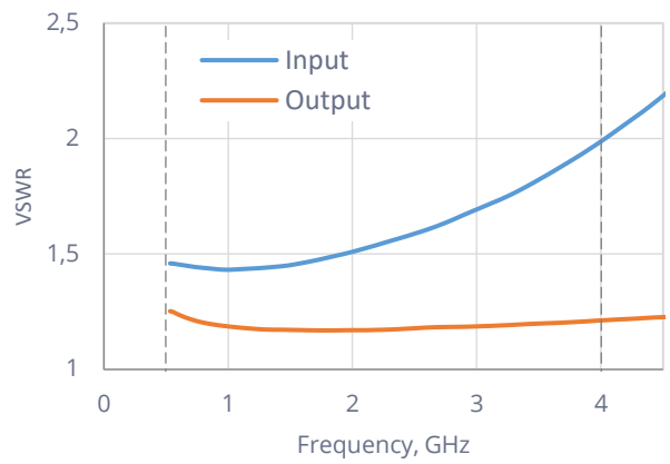
Voltage Standing Wave Ratio (Off)
