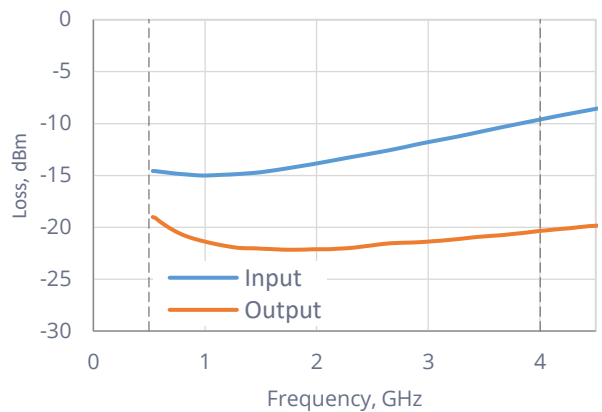
Return Loss (Off)
