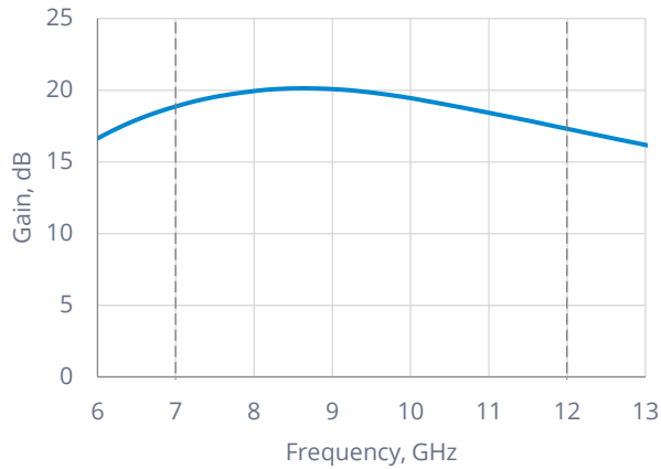
Small Signal Gain ( P_{IN} = -20\text{dBm} )
