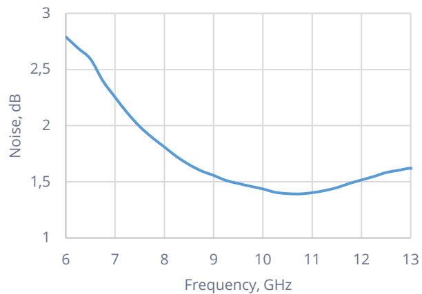
Noise Figure
