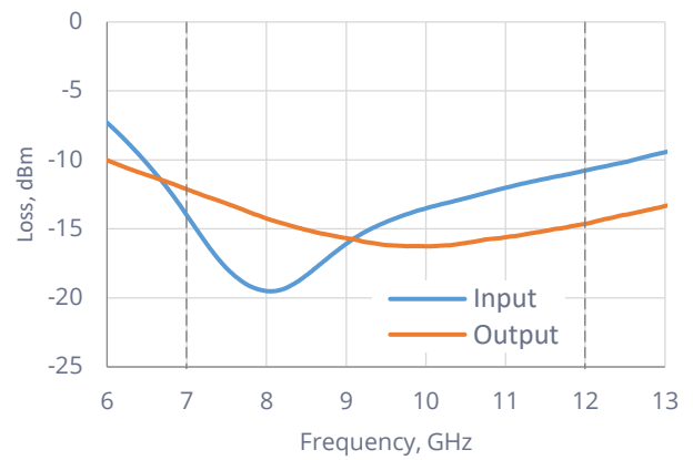
Return Loss
