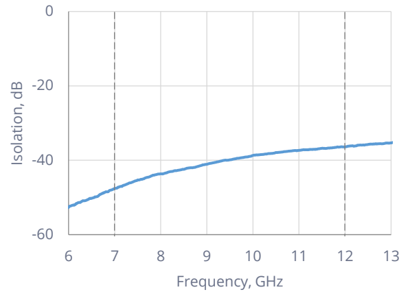
Reverse Isolation
