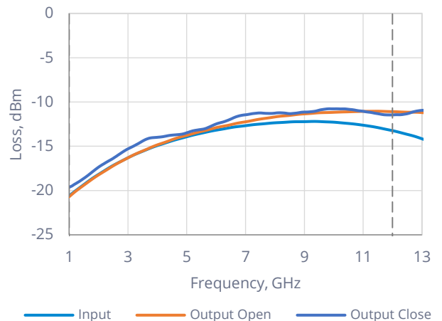
Return Loss ( V_{\text{CONTROL}} = 22\text{V} )
