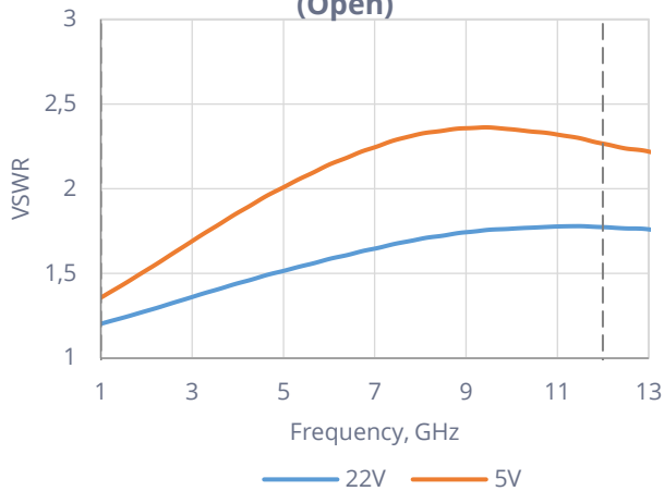
Input Voltage Standing Wave Ratio
