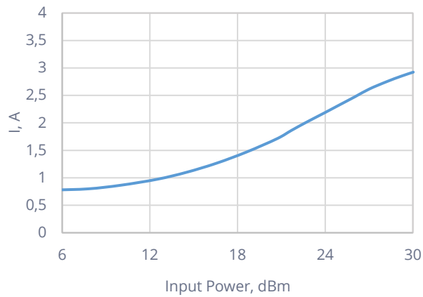
I D vs. P INPUT (frequency point = 10GHz)
