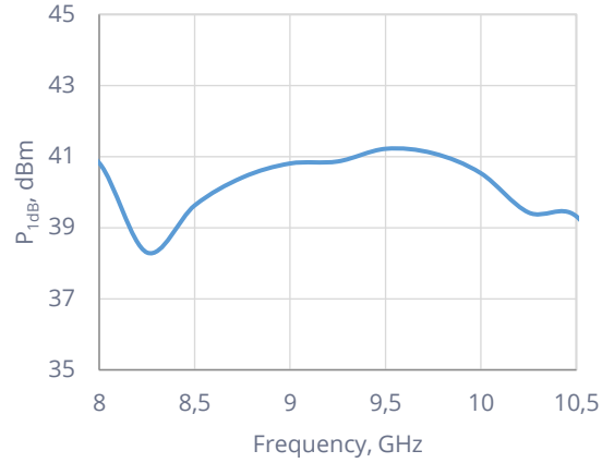
P1dB Compression
