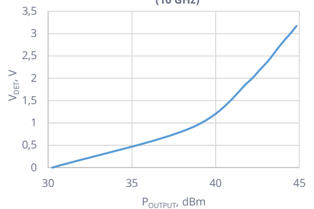
Detector Voltage Output vs. P OUTPUT (10 GHz)
