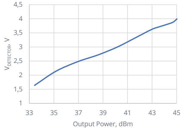
V DETECTOR vs. Output Power
