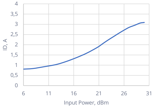
I DRAIN vs. Input Power
