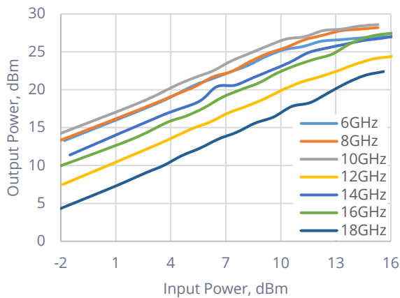
Power Output vs. Input
