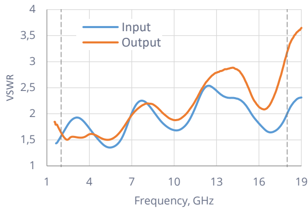
Voltage Standing Wave Ratio
