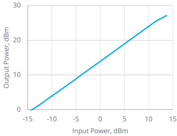
Compression at 4 GHz
