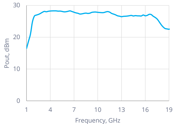
Output Power Saturation ( P_{IN} = 14\text{ dBm} )
