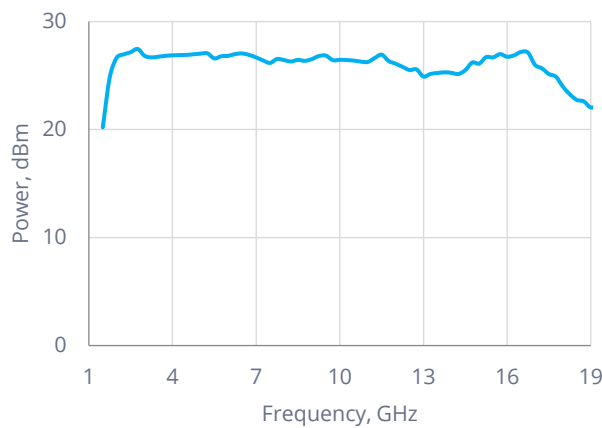
Output P1dB compression
