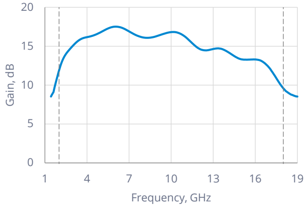
Small Signal Gain ( P_{IN} = -20\text{dBm} )
