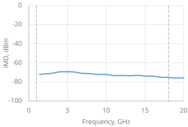
IMD ( P_{IN} = -20 dBm)
