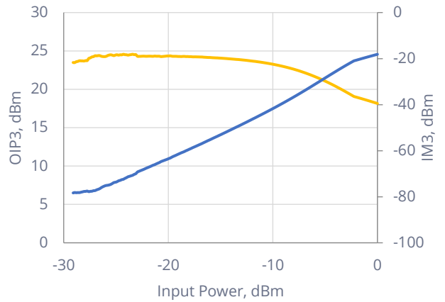
OIP3 & IM3 vs. Input Power
