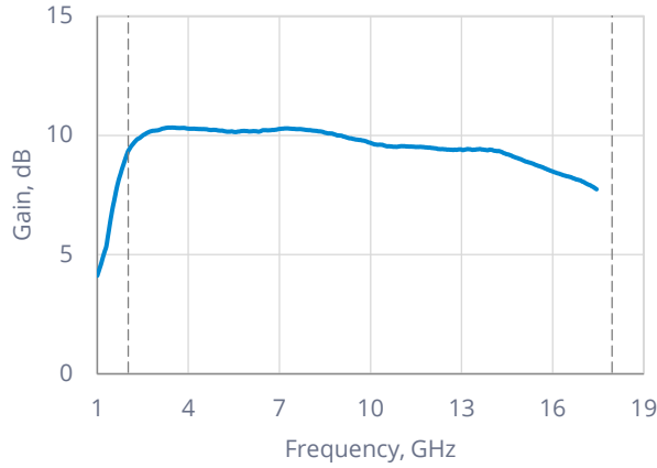
Small Signal Gain ( P_{IN} = -20\text{dBm} )
