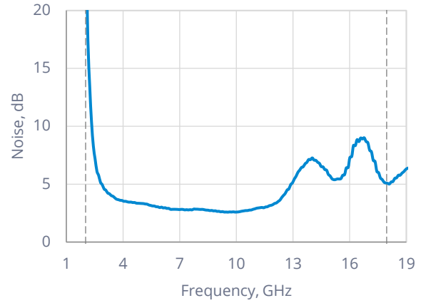
Noise Figure
