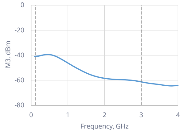
IM3 ( P_{IN} = -10\text{ dBm} )
