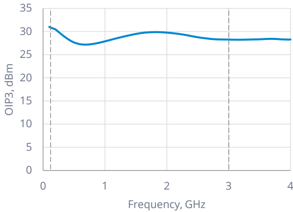
OIP3 ( P_{IN} = -10\text{ dBm} )
