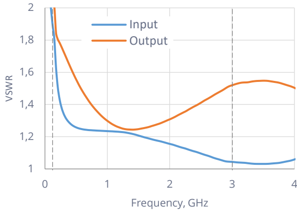
Voltage Standing Wave Ratio
