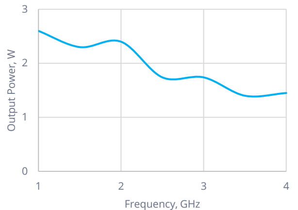
Output Power
