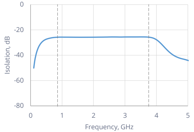
Reverse Isolation
