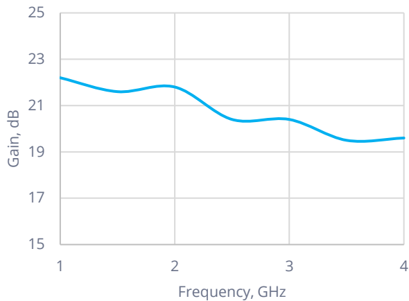
Large Signal Gain ( P_{IN} = 12\text{ dBm} )
